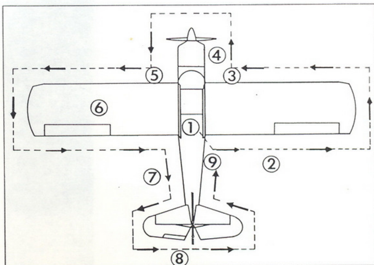
FIGURE 3-1 PREFLIGHT INSPECTION
