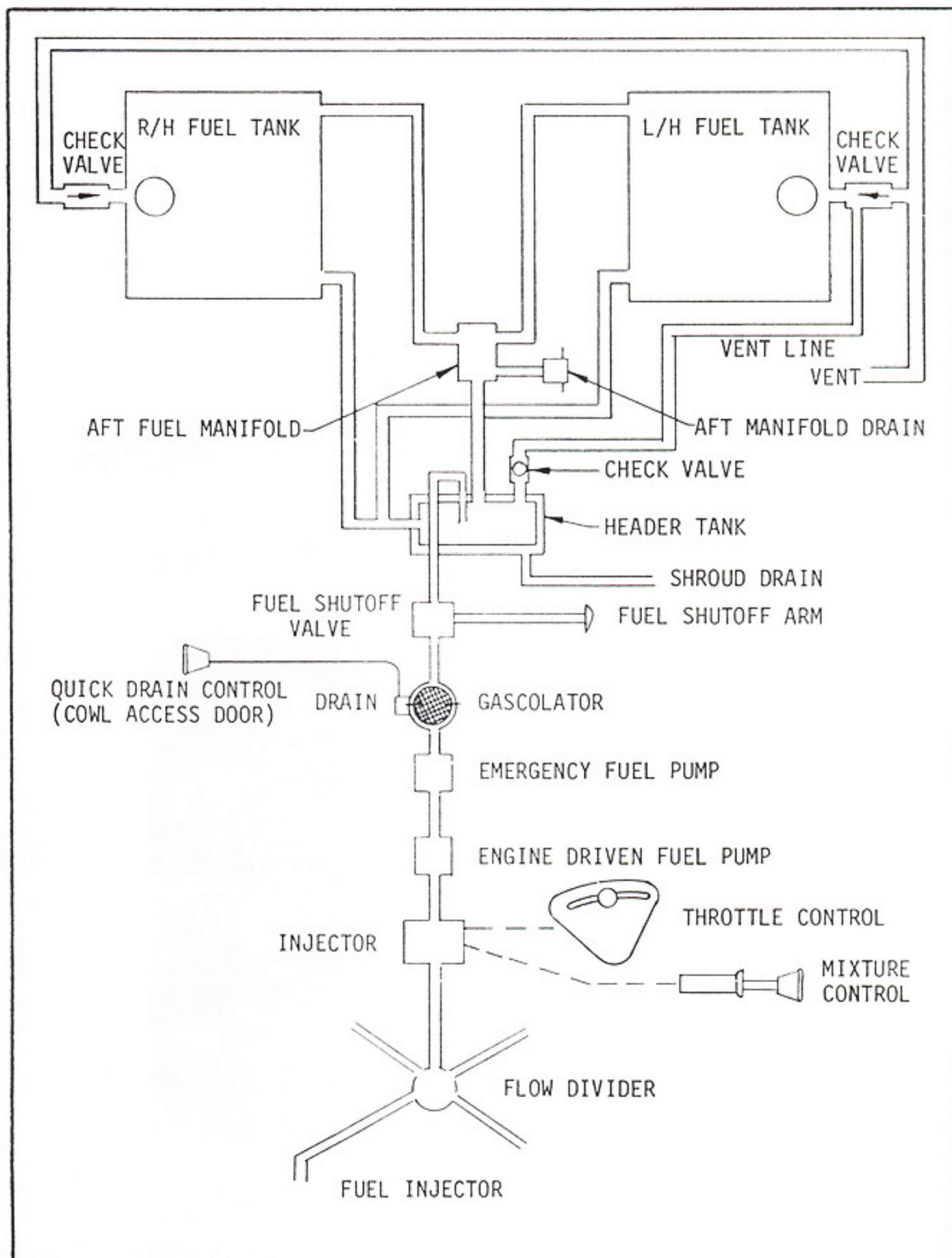
FIGURE 6-2 FUEL SYSTEM SCHEMATIC
