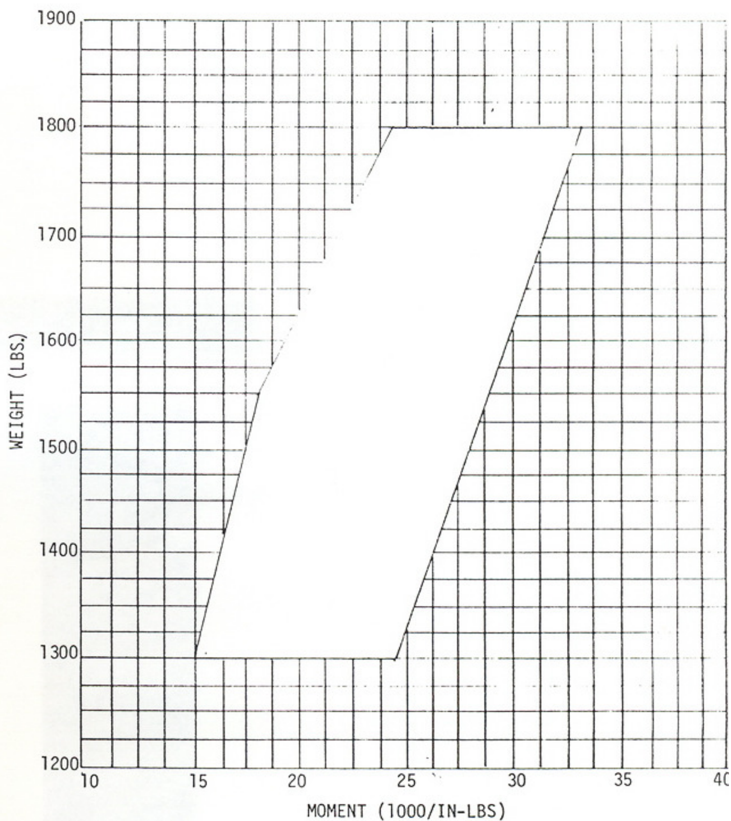
FIGURE 5-4 SUPER DECATHLON WEIGHT AND BALANCE FLIGHT ENVELOPE
