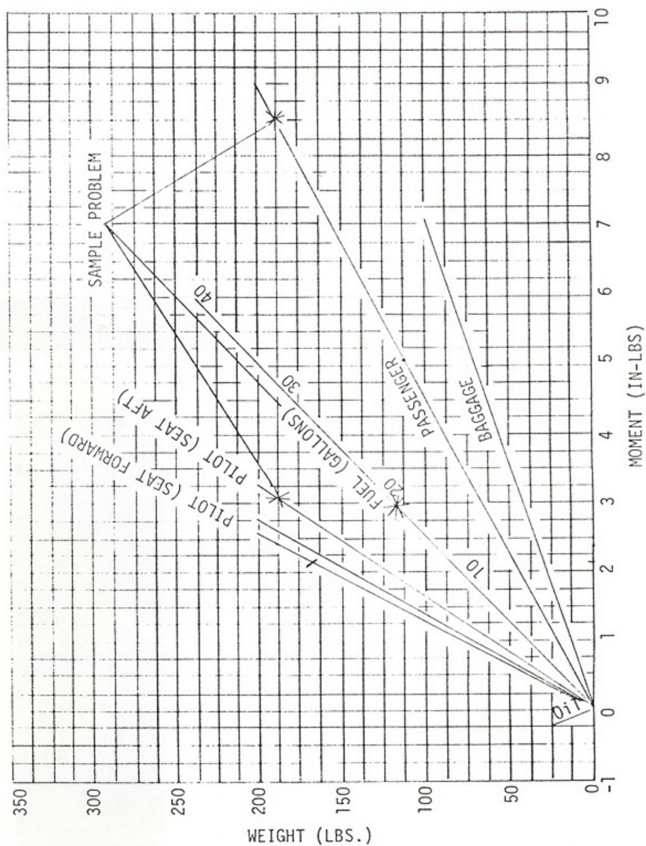
FIGURE 5-2 LOADING GRAPH (All Decathlon Models)
